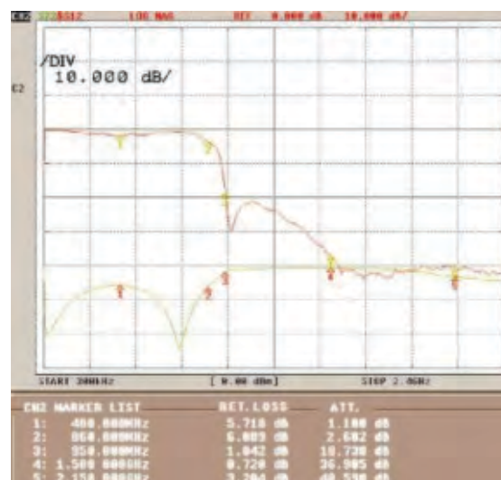
Top TV A/F response and return loss
